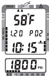
Fig. 40 - Secondary Display
