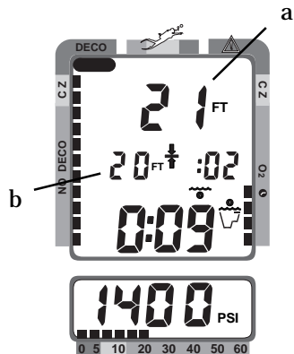
Fig. 65 - Managing a Decompression Stop
