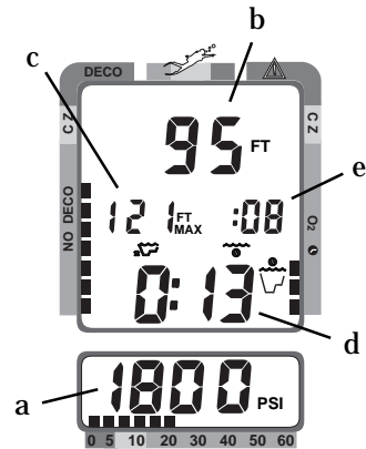
Fig. 11 - Pressure/Depth/Time Displays
