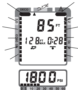
Fig. 71 - Gauge Mode (underwater)
