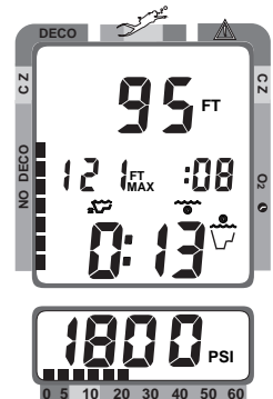
Fig. 31 - Dive Mode (FO2 Set for 'Air')
