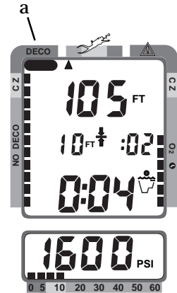
Fig. 42 - Entering Into Decompression Mode
