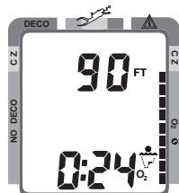
Fig. 36 - Oxygen Control
