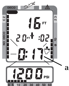
Fig. 67 - Delayed Violation (> 5 minutes above Stop)
