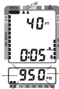
Fig. 63 - Breathing Gas Time Remaining (5 minutes)
