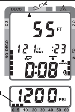
Fig. 10 - Breathing Gas Time Remaining
