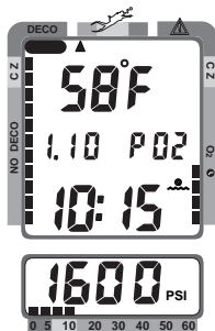
Fig. 61 - Secondary Display
