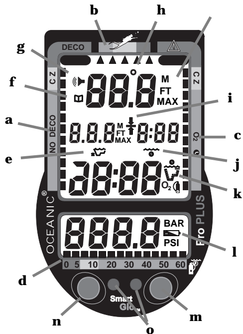
Graphic Interface Legend
