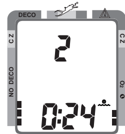
Fig. 47 - Surface Mode (first 2 hours)
